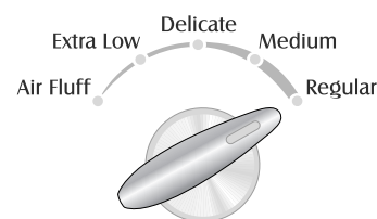
Infinite Temperature
